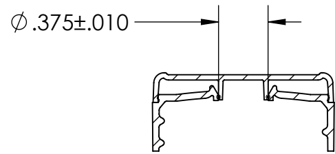
SECTION A-A "OPTIONAL ORIFACE SIZE"
